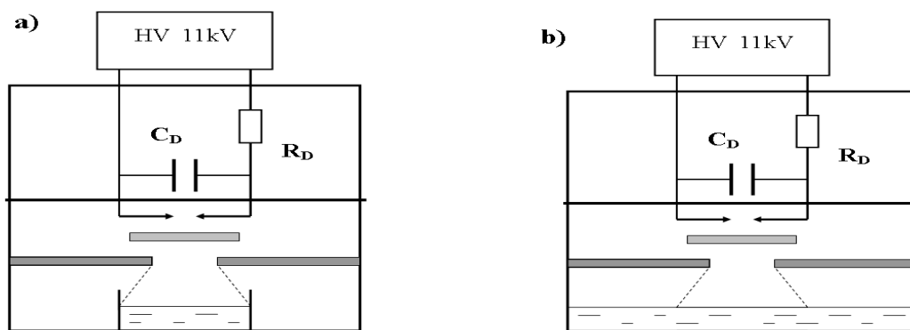
Figure 1: Experimental setup: a) irradiated sample 5 ml; b) irradiated sample 50 ml.
