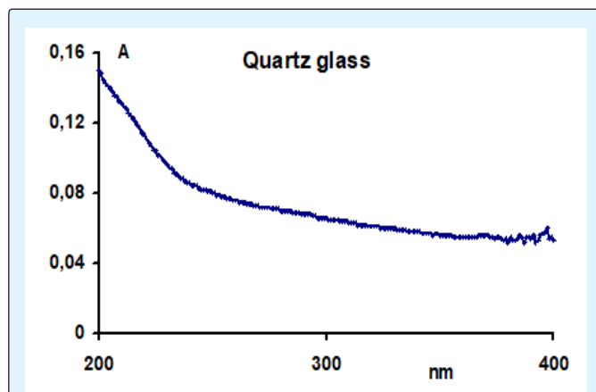
Figure 2: Absorbance of quartz glass 2.3 mm thickness, used in experiment.
