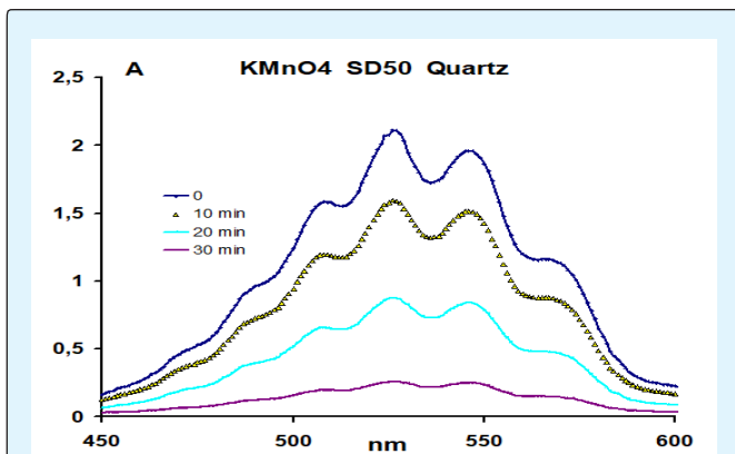
Figure 7: Change in absorption spectrum of \text{KMnO}_4 solution after treatment by radiation of generator SD50 through quartz glass.
